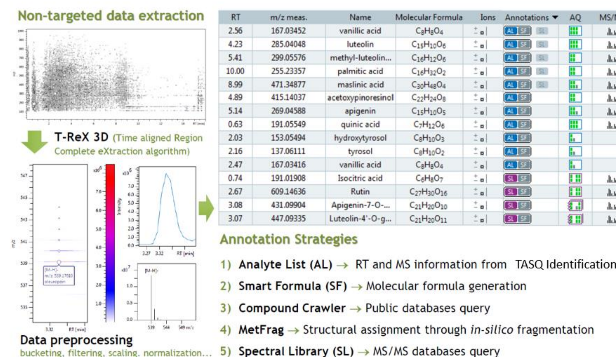
Fig. 4: Workflow for the identification of 'unknown unknowns' with MetaboScape
